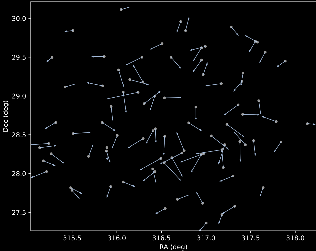
APOGEE DR17 Cluster 1 Proper Motion Vectors (n=85)
