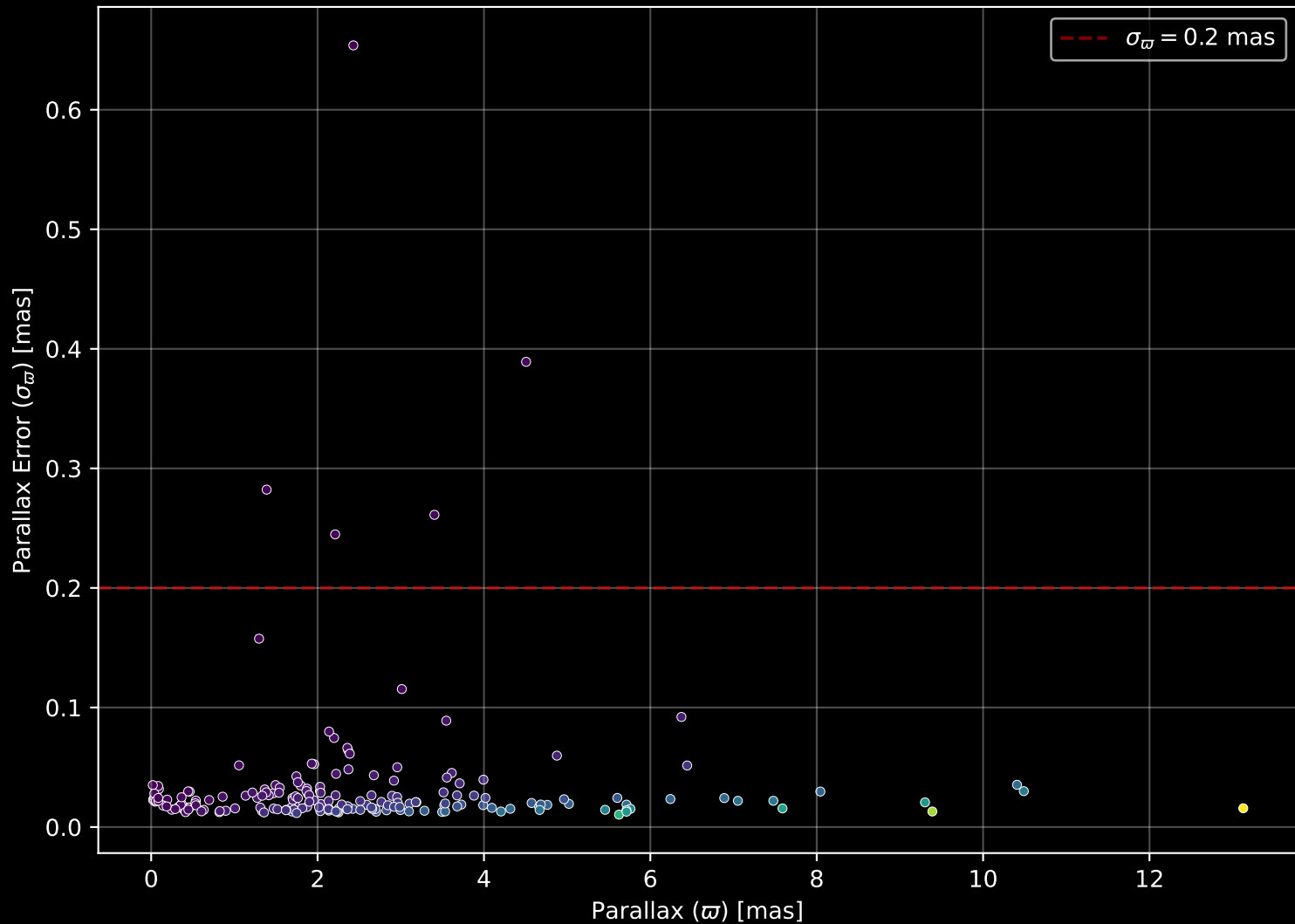
APOGEE DR17 Field: [042+68_btx] Parallax Quality (n= 187)
