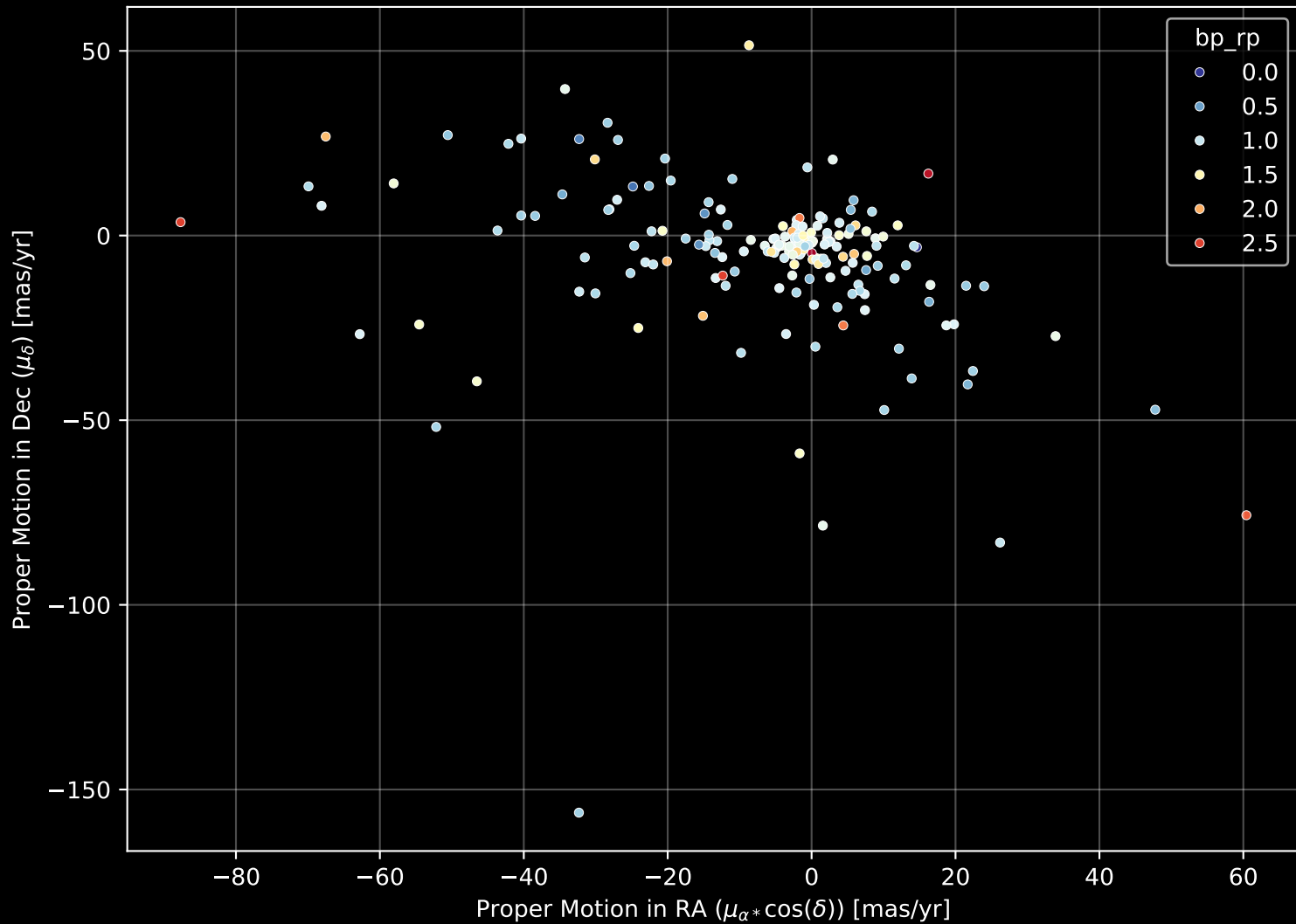
APOGEE DR17 Field: [042+68_btx] Proper Motion Diagram (n= 187)
