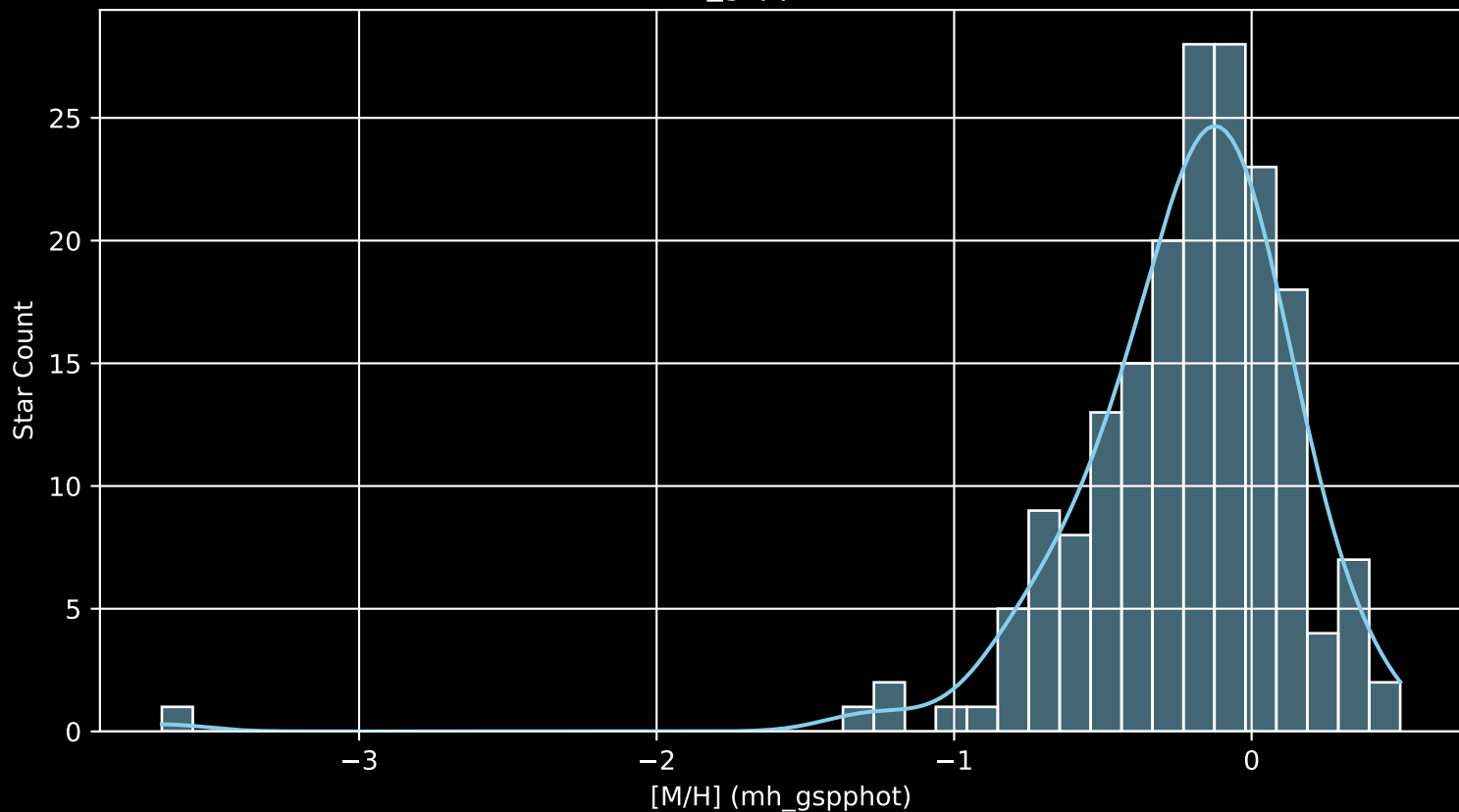
APOGEE DR17 Field: [042+68_btx [M/H] (mh_gspphot) (n= 186)
