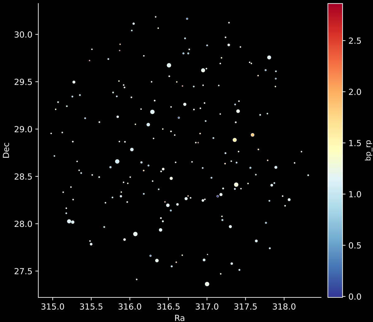
APOGEE DR17 Field: [042+68_btx] Stars: 187
