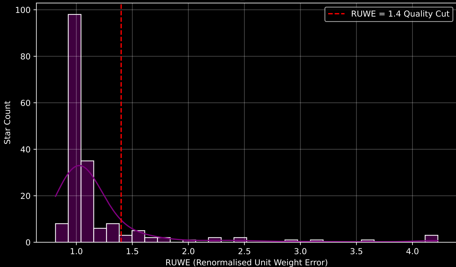
GAPOGEE DR17 Field [042+68_btx] RUWE Distribution (n= 178)
