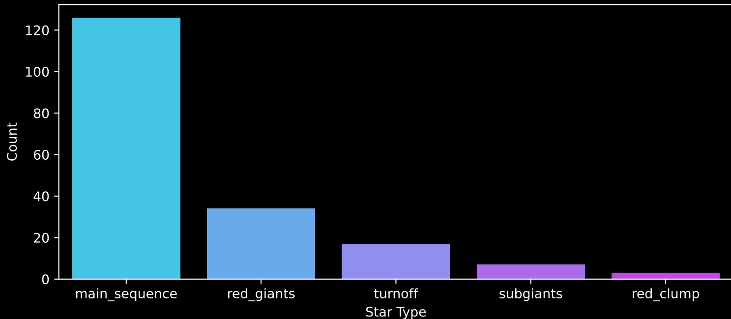
APOGEE DR17 Field: [042+68_btx] Count plot of Star Type
